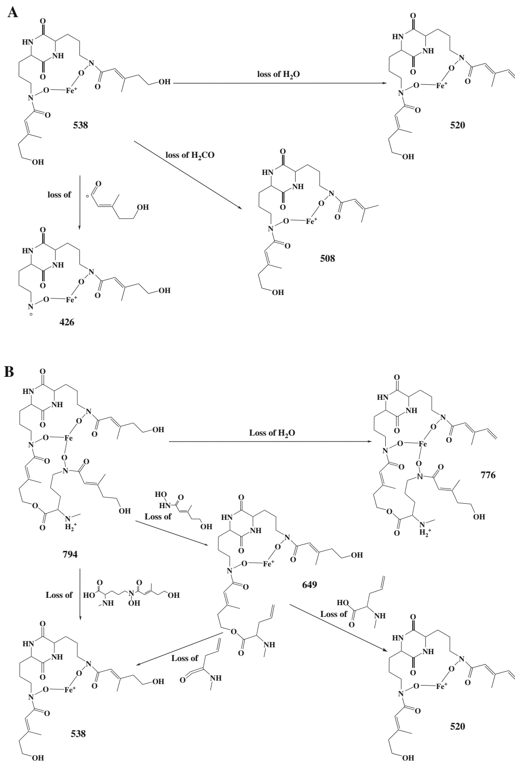
Fig. 7 Fragmentation scheme of iron chelate of dimeric acid (A) or N^\alpha -methyl coprogen B (B) by ESI+-MS
